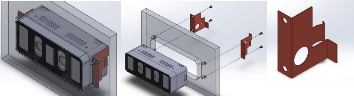
Type C : Auto clamp bracket top and bottom
