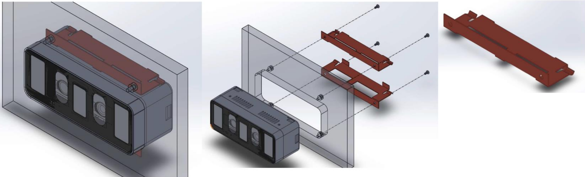
Type B : Side mount using a bracket
